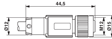
M12 x 1 socket, straight, shielded
